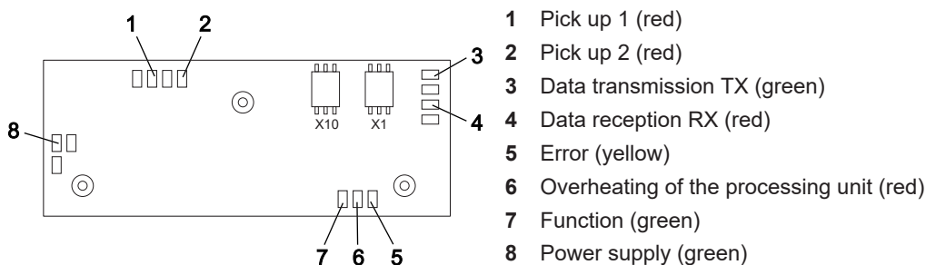
Fig. 9: Status LEDs
